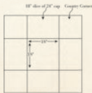
Cap for 38" Pier: Size: 42" square Note: Leave 18" square in center open for plantings or cover with 24" pier cap. (24" pier cap for center may need to be glued at the joints ahead of time and allowed to set up prior to installation.)
