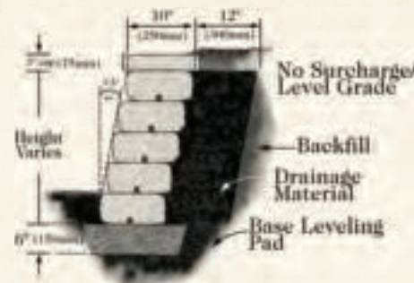
Gravity Wall – Setback Detail 9.5° + Batter
